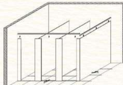
6) Set the top rail in place and ensure it is properly aligned
