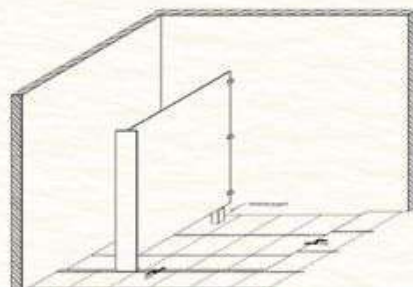
5) Position and secure the dividing panel to the wall using temporary supports, then continue the same procedure for the remaining panels.
