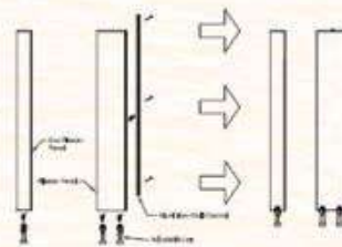
4) Preparation adjustable leg & wall angle secure on front pilaster
