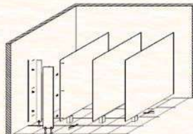
6) Secure the pilaster to the dividing panel and continue with the same installation sequence until finished
